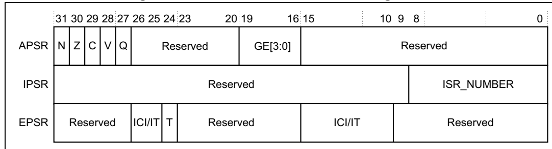
Figure 3. APSR, IPSR and EPSR bit assignment
