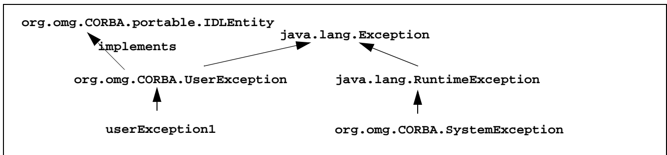
Figure 1-1 Inheritance of Java Exception Classes
